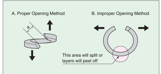
Fig. 5 Proper Installation
