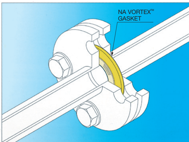
●The above diagram shows the cross-sectional view of the flanges and pipework.
