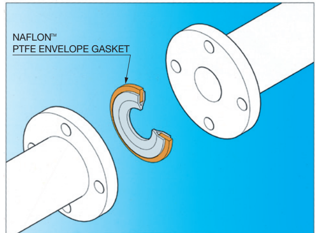
● The above diagram shows the cross-sectional view of the gasket.
